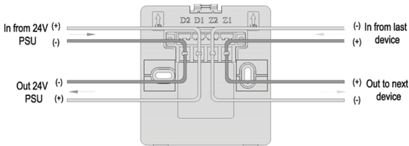
Fig.2 Wiring Details
