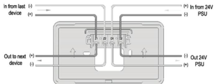
With External Supply Wiring Details
