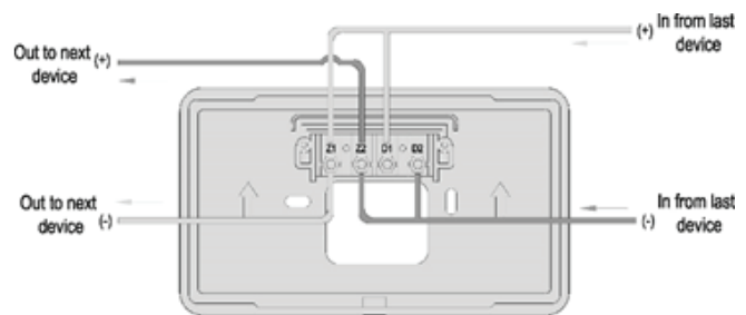
Loop Powered Wiring Details
